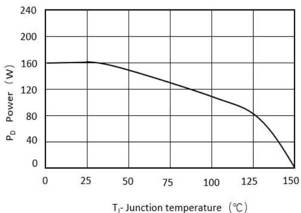
Figure 7. Power De-rating
