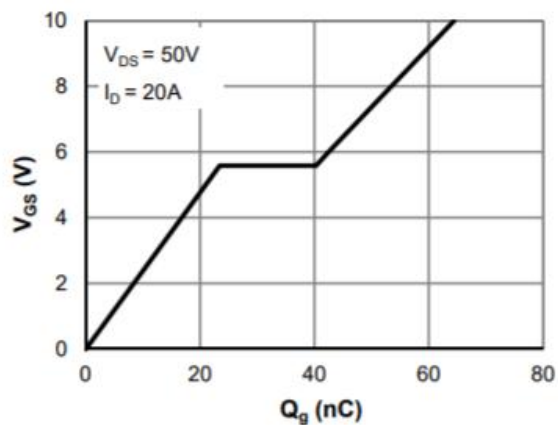
Figure 5. Gate Charge
