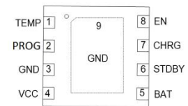
DFN2*2-8L
