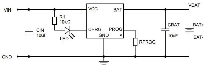
Figure 1. Without absorption circuit
