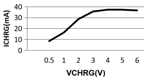
CHRG Pin I-V Curve (Strong Pull-Down State)
