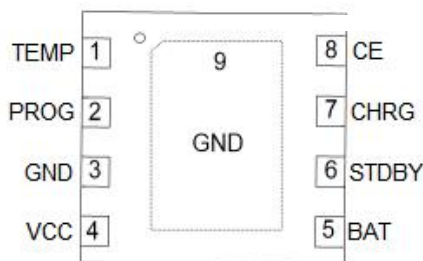
DFN2*2-8L
