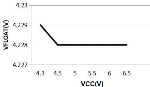
Regulated Output (FLOAT) Voltage VS Supply Voltage
