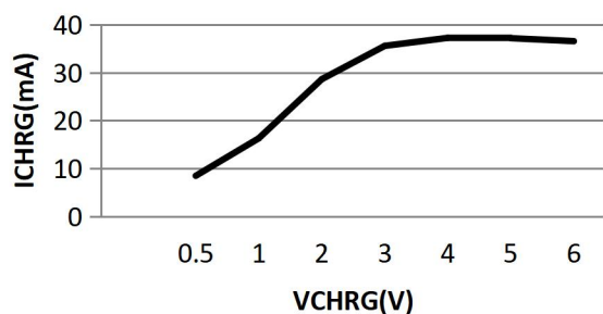
CHRG Pin I-V Curve (Strong Pull-Down State)
