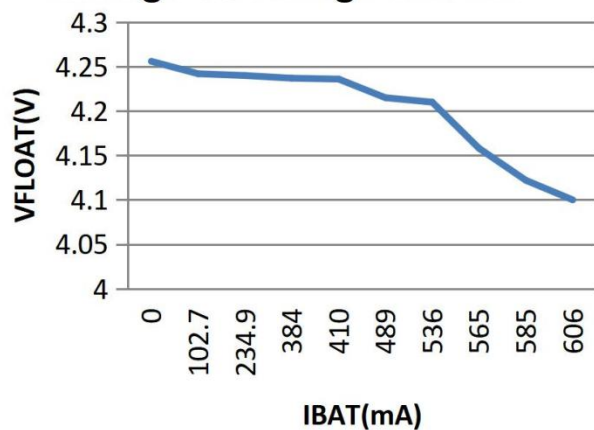
Regulated Output (FIOAT) Voltage VS Charge Current
