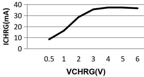
CHRG Pin I-V Curve (Strong Pull-Down State)
