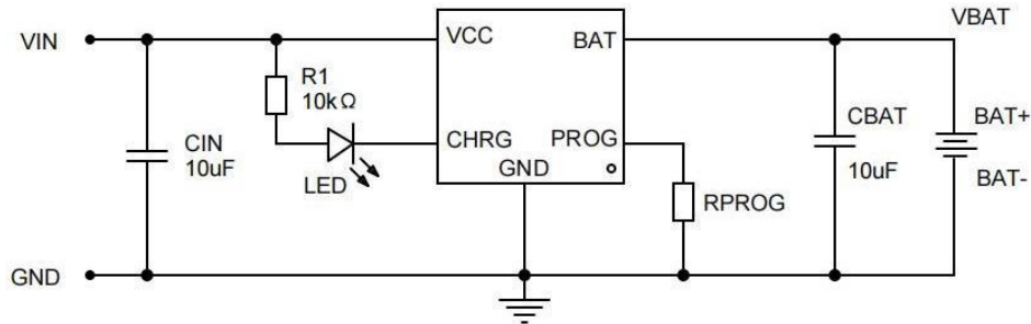
Figure 1. Without absorption circuit
