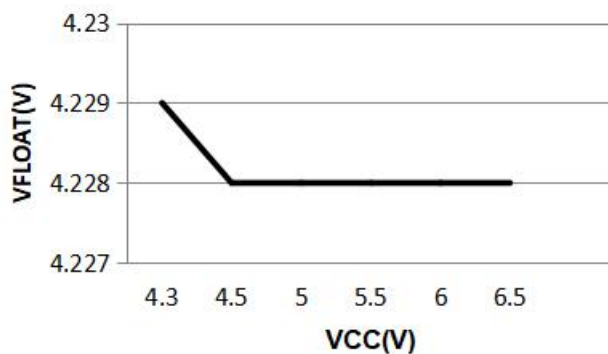
Regulated Output (FLOAT) Voltage VS Supply Voltage
