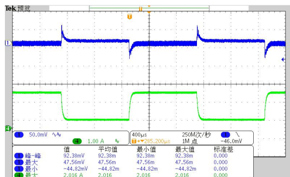
Vin=3.3V, 0.5A to 2A transient waveform (Transient Response)
