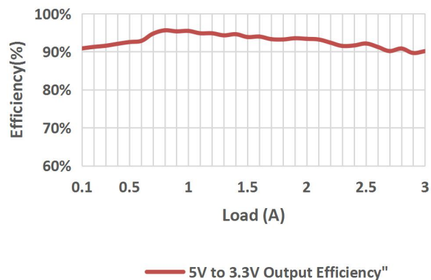
5V to 3.3V Output Efficiency
