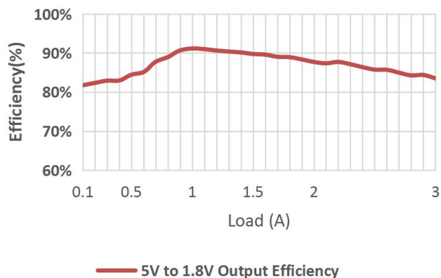
5V to 1.8V Output Efficiency
