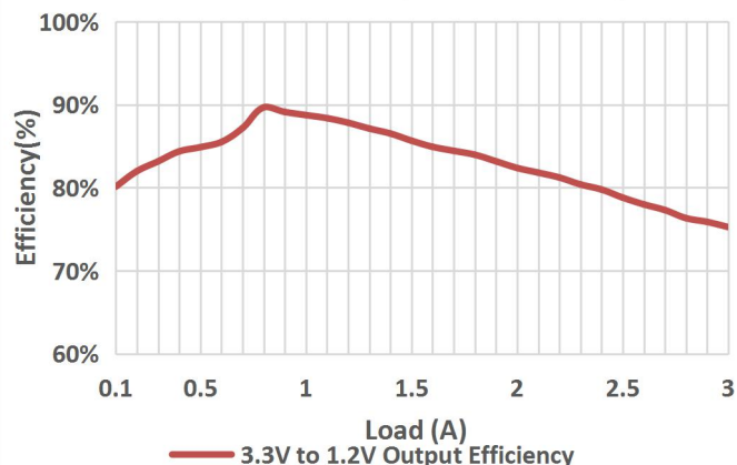
3.3V to 1.2V Output Efficiency
