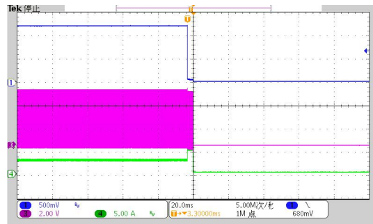
Iload=3A short
