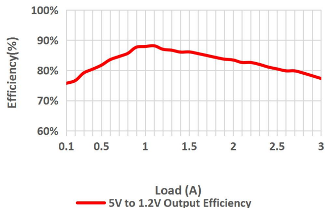
5V to 1.2V Output Efficiency
