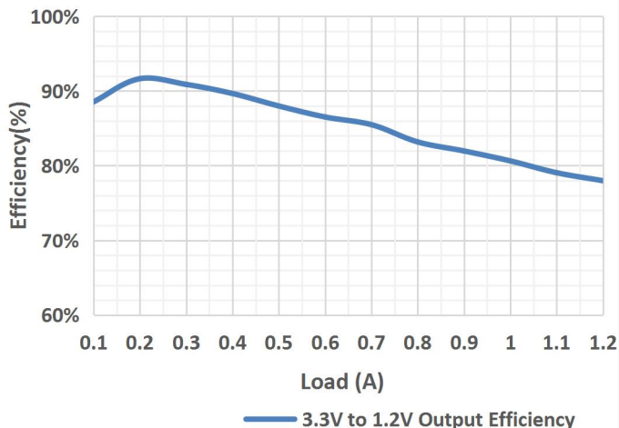
3.3V to 1.2V Output Efficiency
