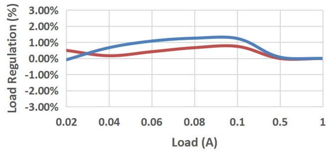
Load Regulation
