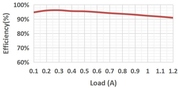
5V to 3.3V Output Efficiency
