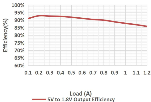
5V to 1.8V Output Efficiency
