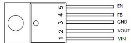
TO-220-5L
