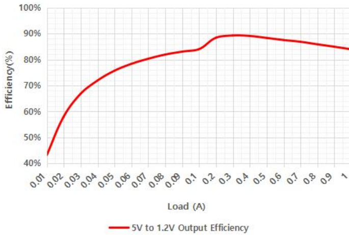
5V to 1.2V Output Efficiency
